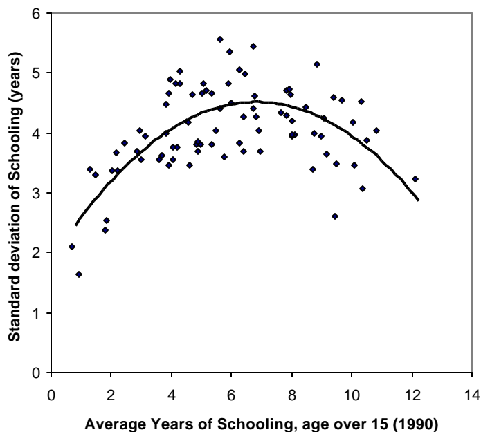
Figure 8. Education Kuznets Curve, Standard Deviation of Schooling, 1990
