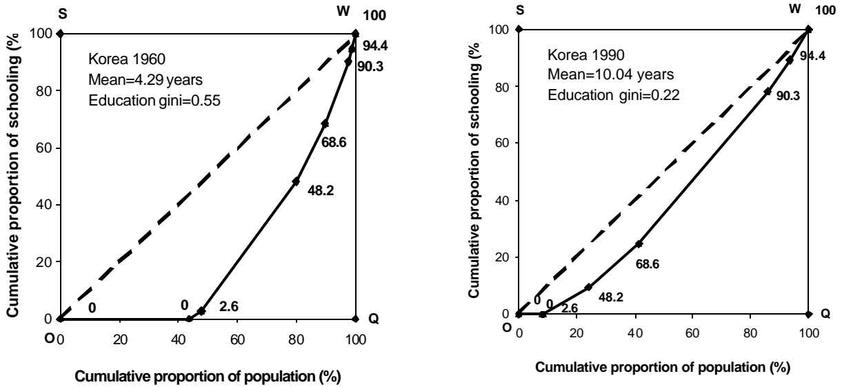
Figure 5 Education Lorenz Curves, Korea, 1960 and 1990
