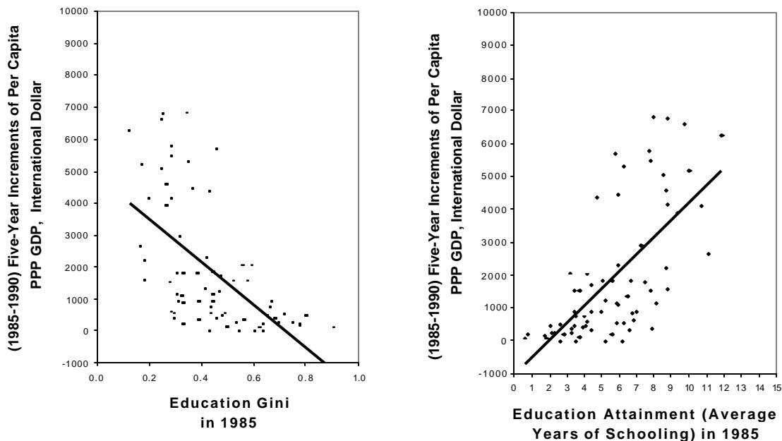
Figure 11. Education Gini, Attainment and per capita PPP GDP Increments
