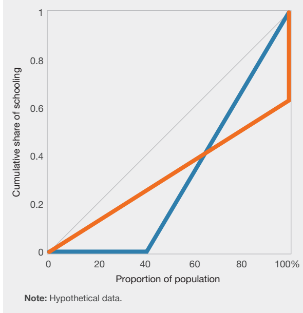
Figure 3.12 Symmetric Lorenz curves for two independent populations with equal Gini coefficients
